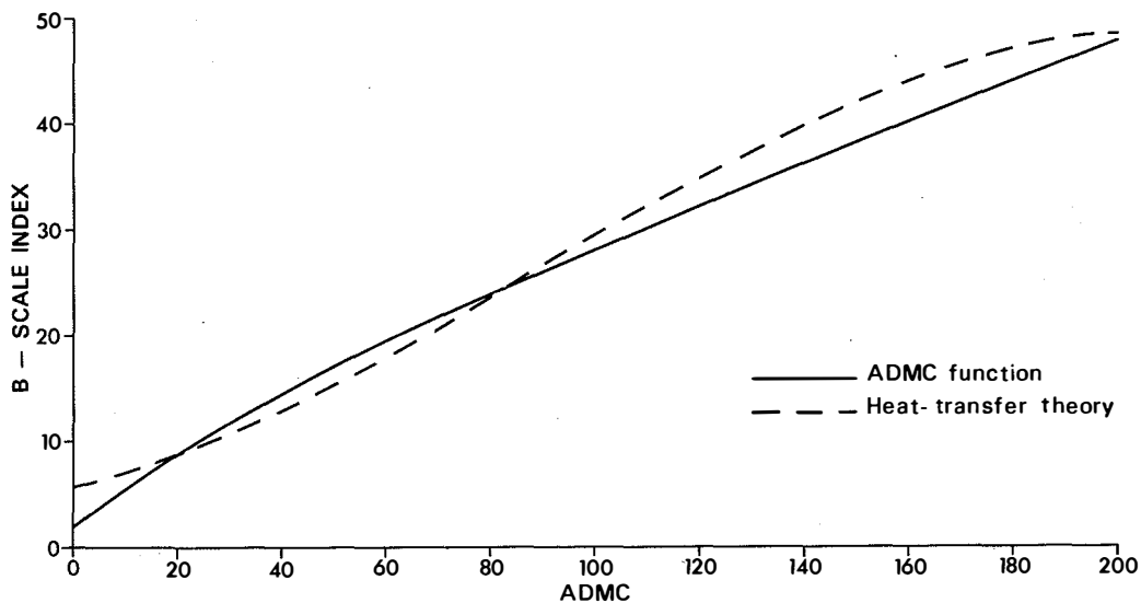
Figure 10. Effect of ADCM on B-scale FWI along with curve based on heat transfer theory.
